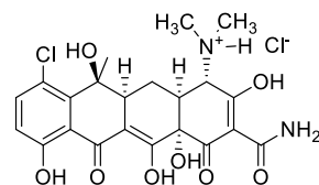
Chlortetracycline hydrochloride
