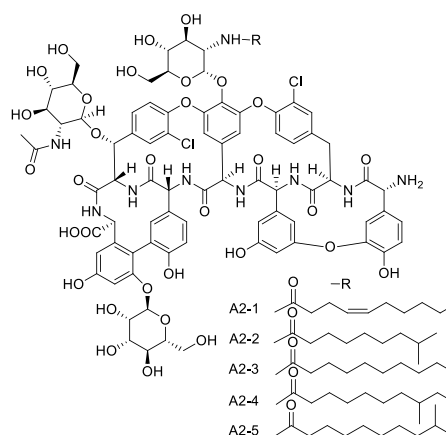
Teicoplanin complex
