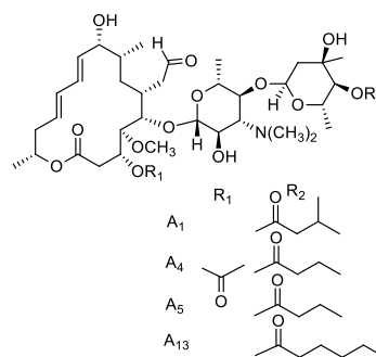
Leucomycin complex
